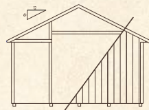
Standard 6'6" Sidewalls - 4 Pitch - No Loft
