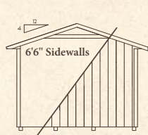
Standard 6'6" Sidewalls - 4 Pitch - No Loft
