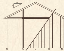
Elite Package 7' Sidewalls - 6 Pitch - Loft
